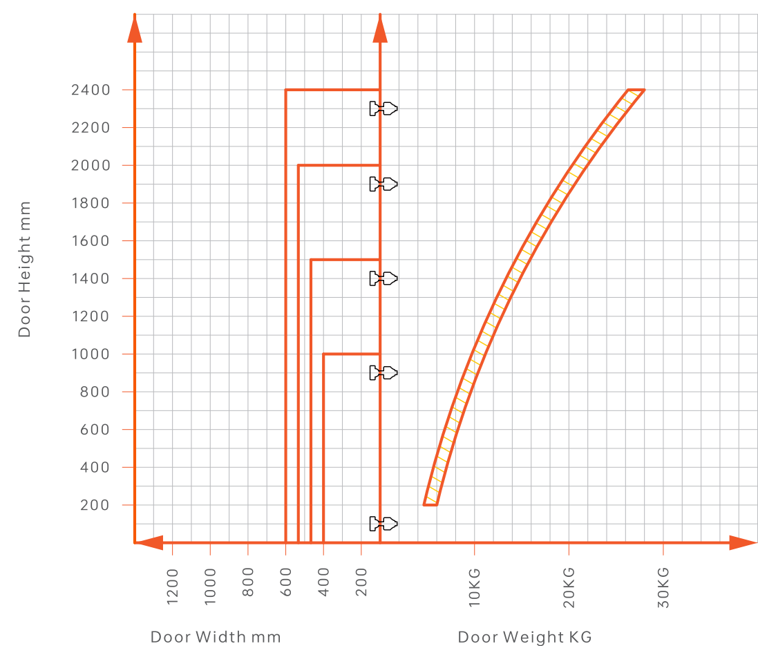
Allowance of Force and the weight of panel calculation sheet
