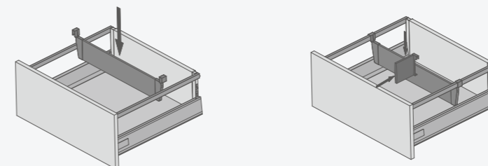
GR cross partition mounting
