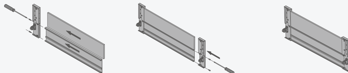
High side inner box drawer with higher side panel mounting
