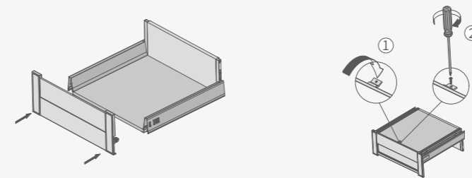
High side inner box drawer with higher side panel mounting
