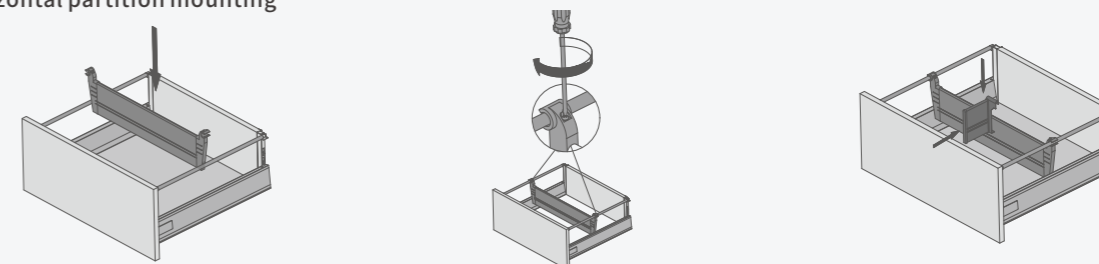
C horizontal partition mounting
