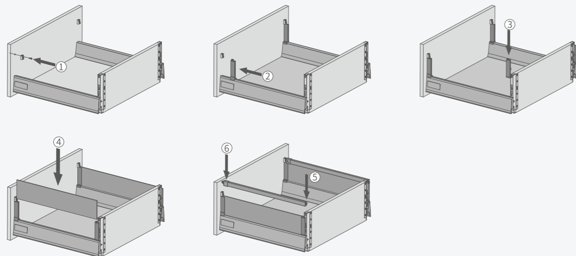
Square bar and higher side panel mounting
