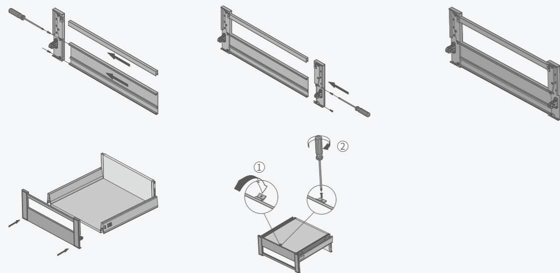
With handrail mounting
